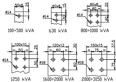
Low voltage terminal
